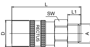
Male Thread
