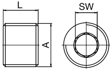
Male Thread tapered, with Socket Pipe
